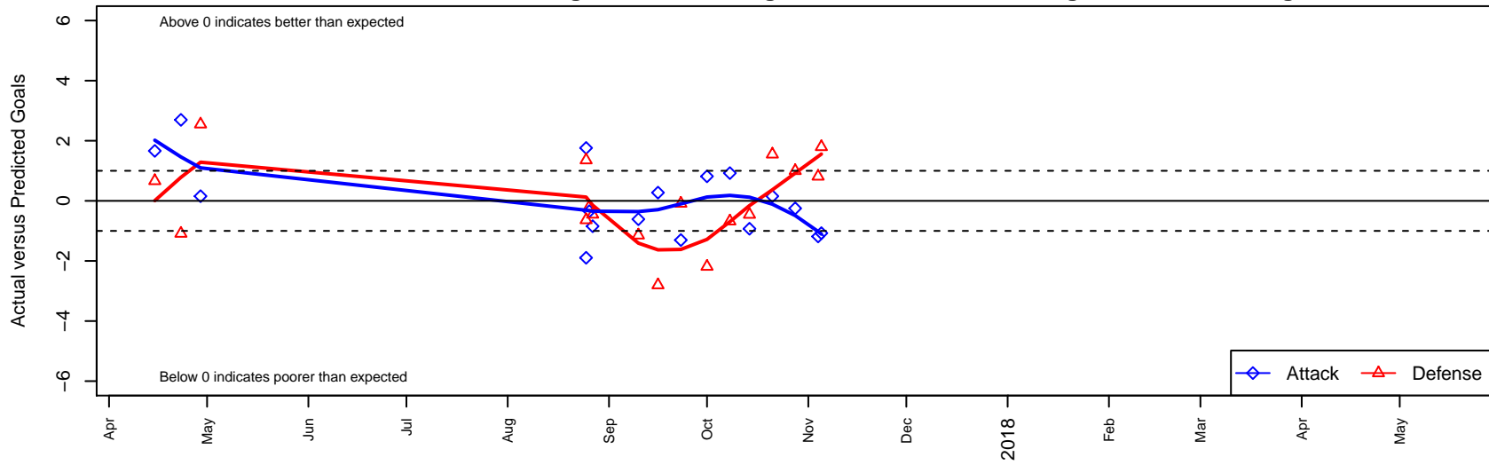
THUSC Fluorine B03 Dots are actual minus expected GF (blue circles) and GA (red triangles). Blue line is smoothed change in attack strength. Red is smoothed change in defense strength.
